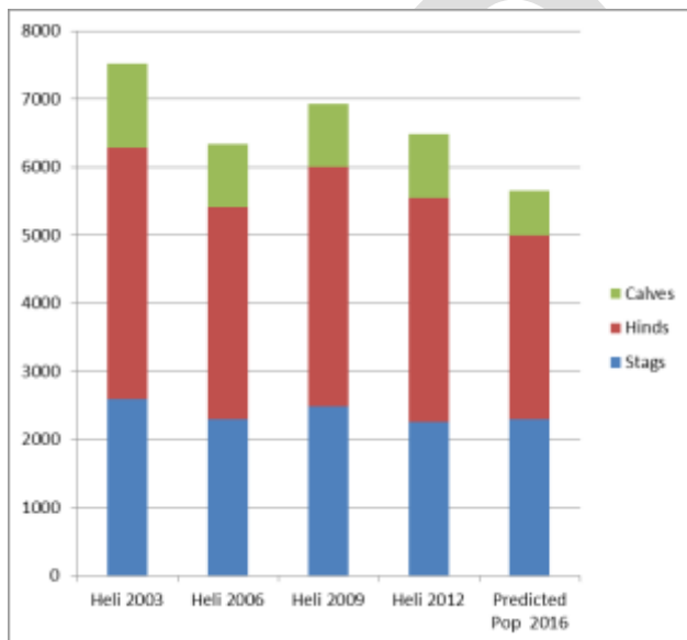
Figure 3: Actual and Predicted Deer Populations
